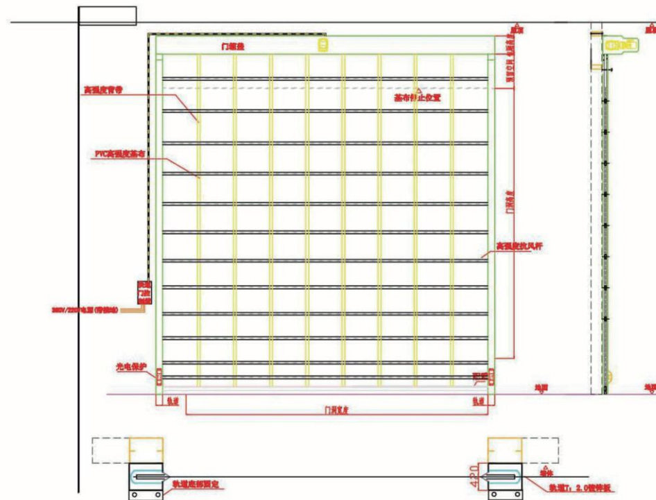
堆积门中装示意图 A schematic diagram of stacking doors
