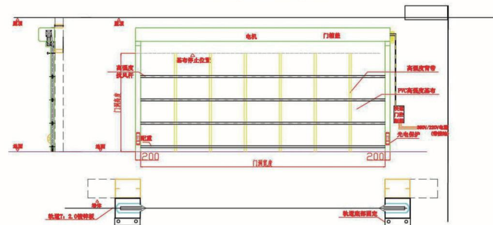
堆积门正装示意图 Schematic diagram of stack door dress
