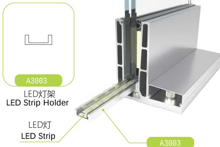
LED灯带 LED Strip
