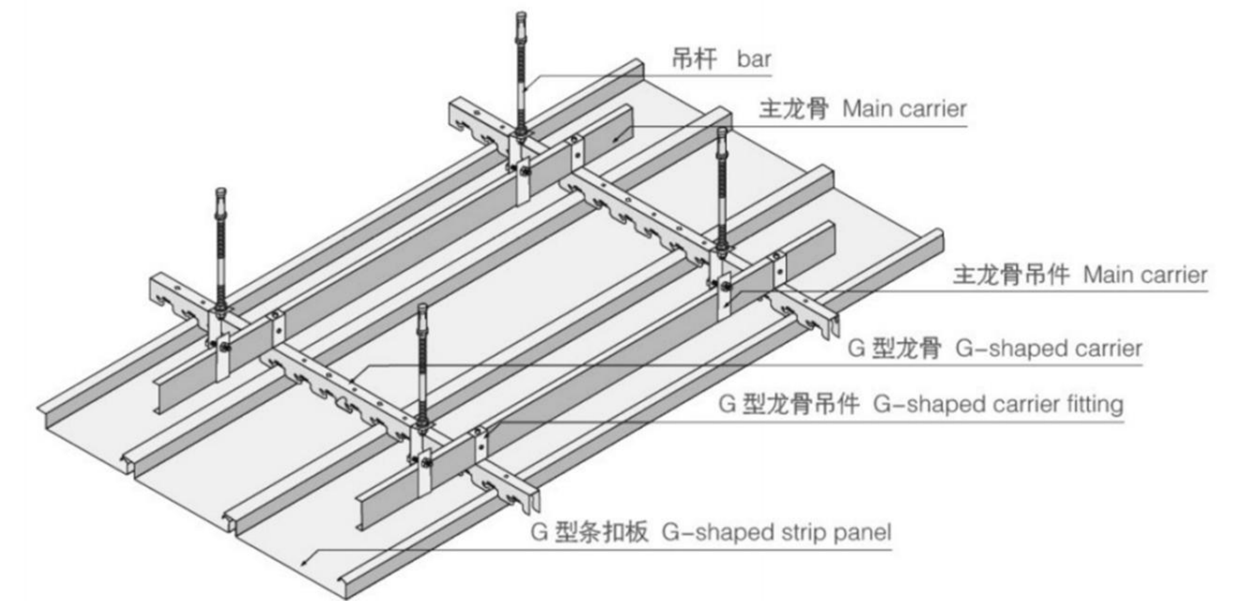
密封条扣有宽 200、300、400mm 等不同规格 Width of the closed strip have sizes of 200, 300, 400mm.
